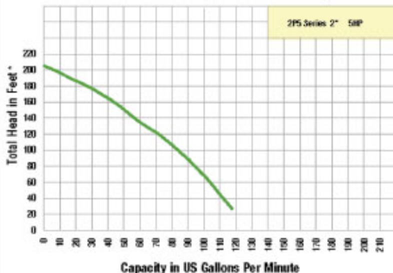
Performance of High Pressure Pumps
